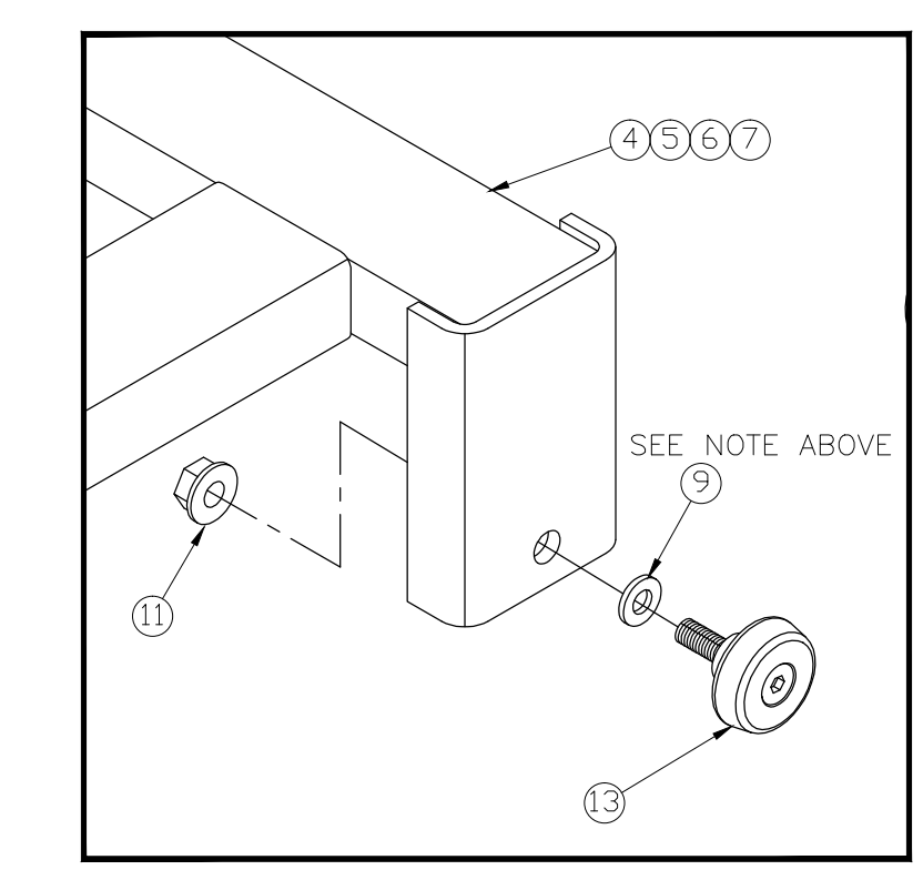
CART 3, 4, 5 & 6 REAR WHEEL CONNECTION DETAIL
