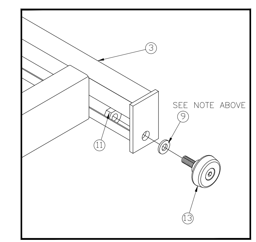
CART 2 WHEEL CONNECTION DETAIL
