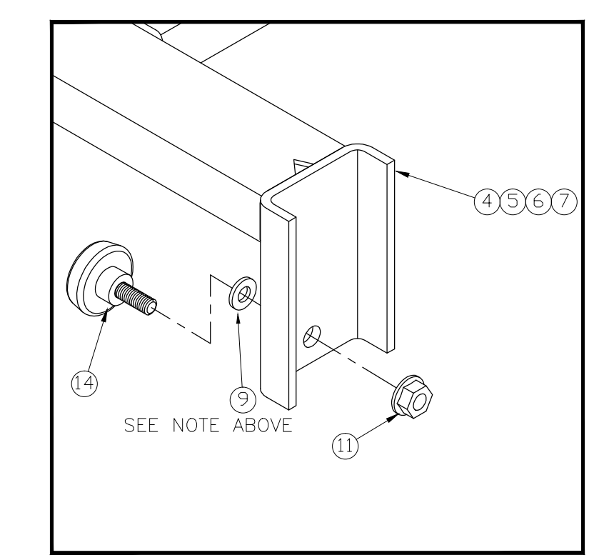
CART 3, 4, 5 & 6 FRONT WHEEL CONNECTION DETAIL
